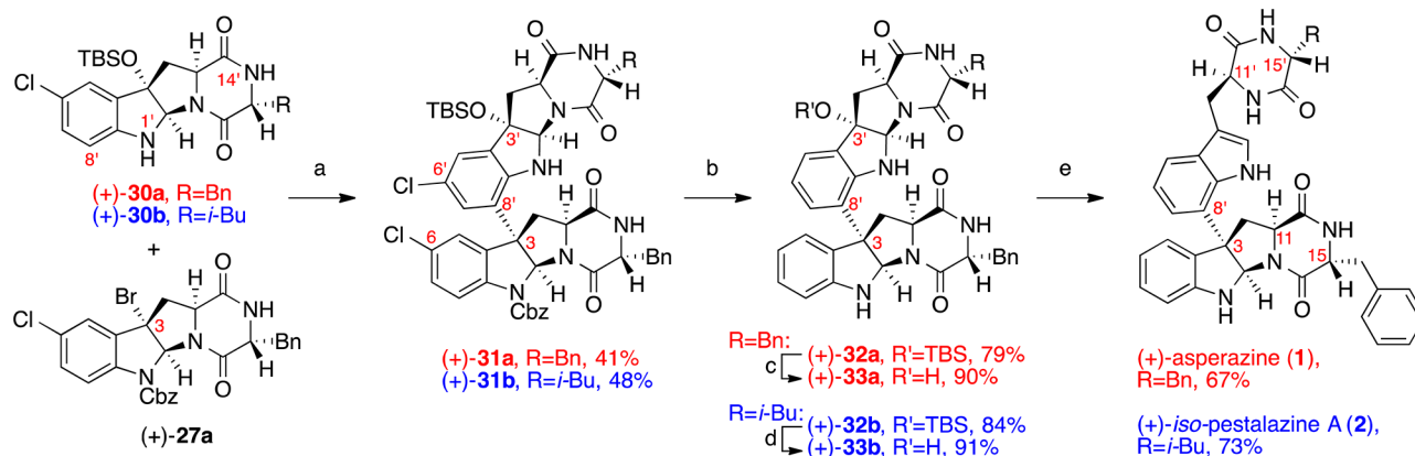
Scheme 6. Friedel–Crafts Reaction and Ring-Opening: Synthesis of (+)-Asperazine (1) and (+)- iso -Pestalazine A (2) 4a
